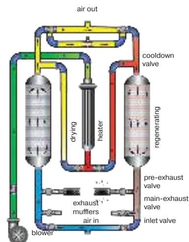
TWB Series Blower Purge
