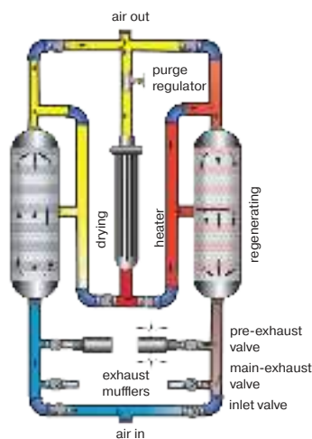
TWP Externally Heated with Patented Multi-Port
