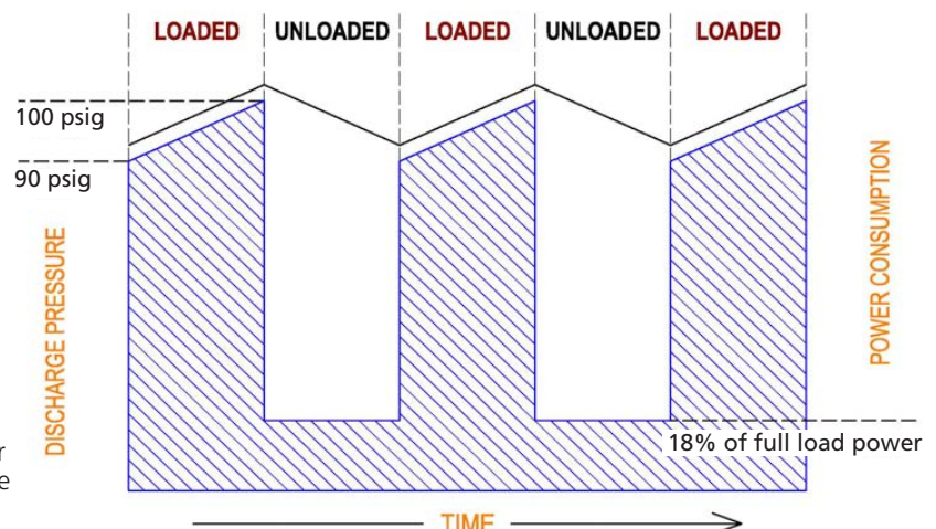
Fixed Speed Power and Pressure Profile
