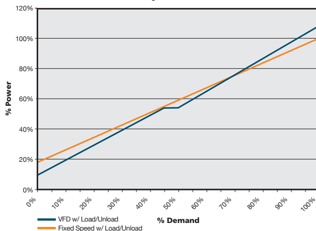
Cost of operation Fixed Speed vs. VFD
