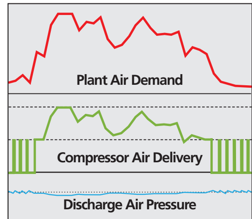
VFD Flow and Pressure Profile
